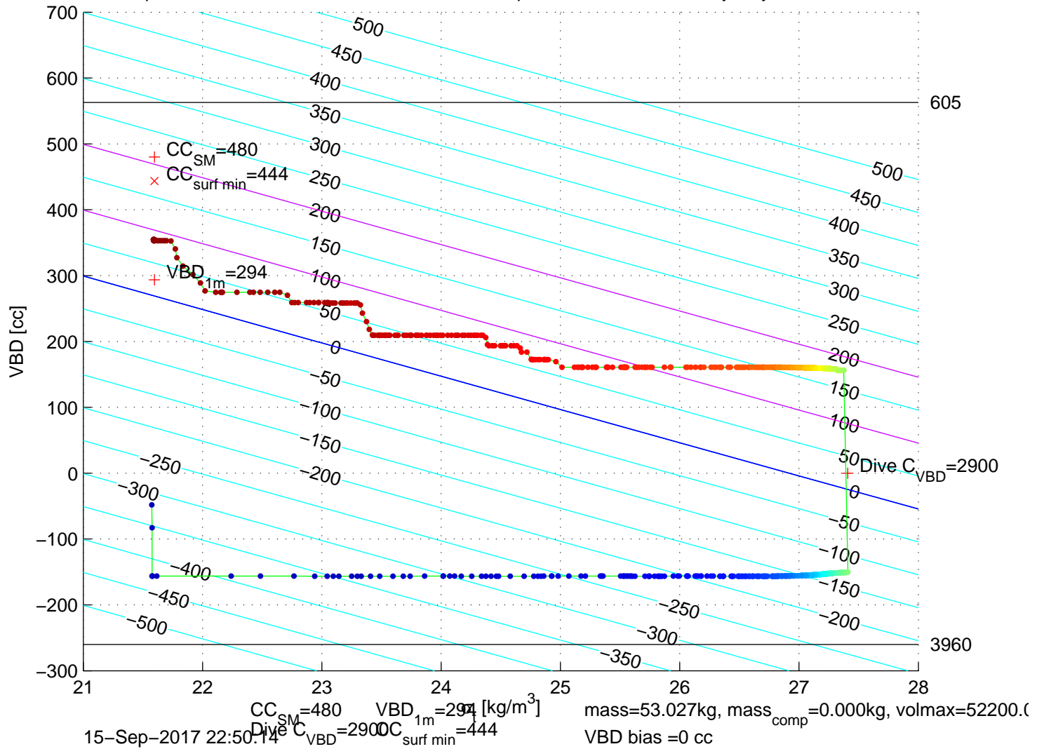
p6300503: SG630 Mission 7 Jul 2017 15-Sep-2017 23:25:09Z – buoyancy contoured
