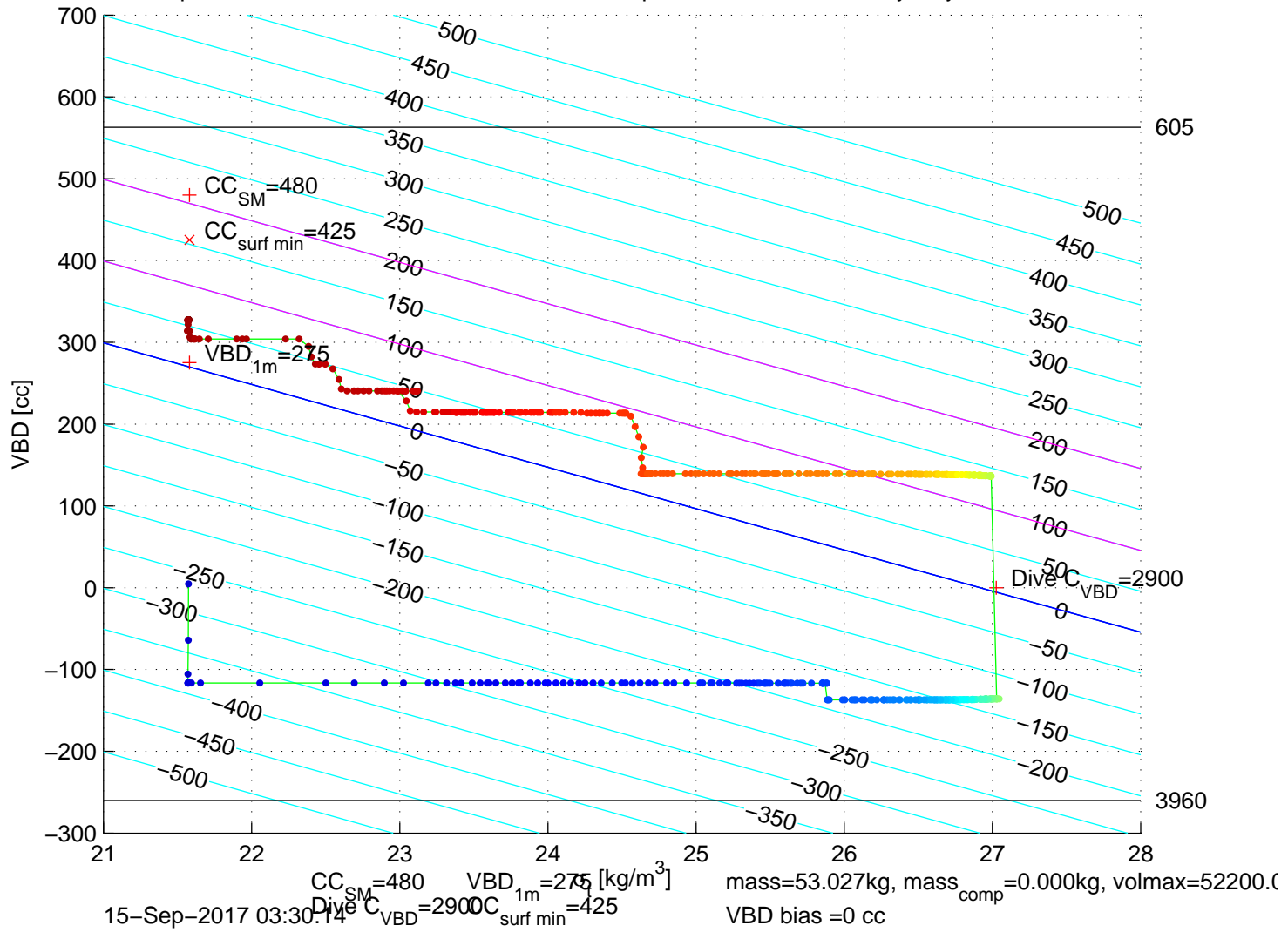
p6300496: SG630 Mission 7 Jul 2017 15-Sep-2017 05:16:19Z – buoyancy contoured
