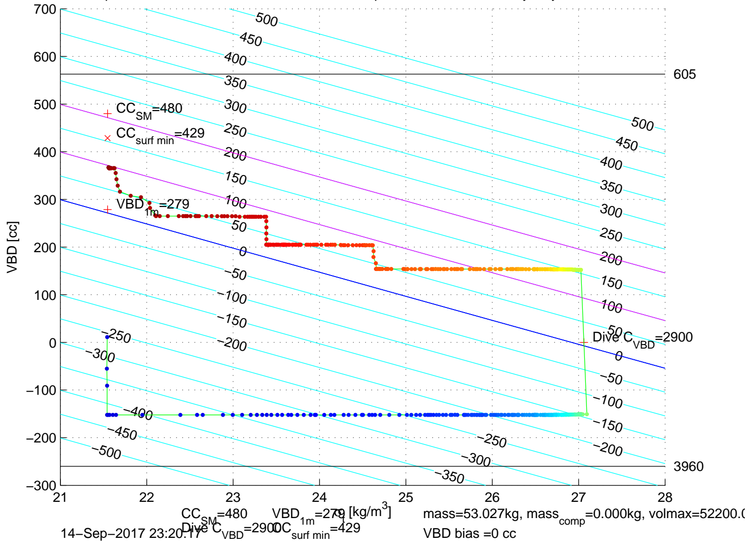
p6300494: SG630 Mission 7 Jul 2017 15-Sep-2017 01:04:05Z – buoyancy contoured
