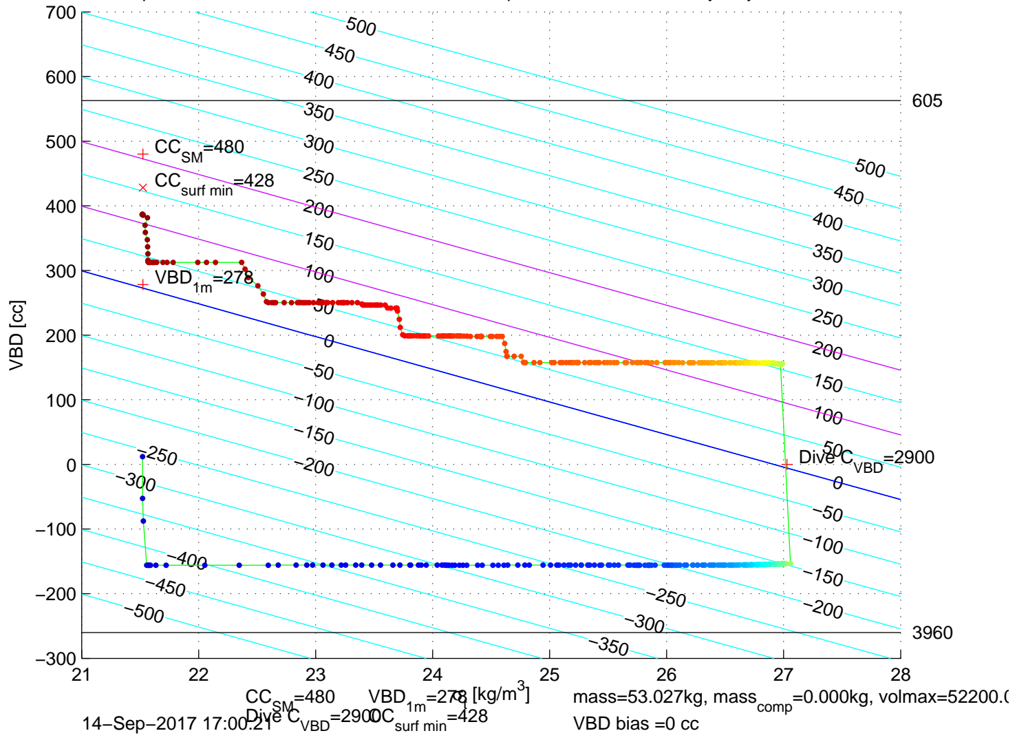
p6300491: SG630 Mission 7 Jul 2017 14-Sep-2017 18:29:55Z – buoyancy contoured
