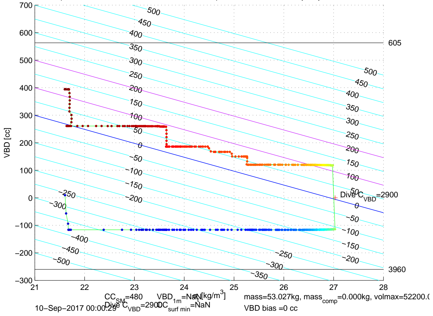
p6300441: SG630 Mission 7 Jul 2017 10-Sep-2017 01:38:14Z – buoyancy contoured
