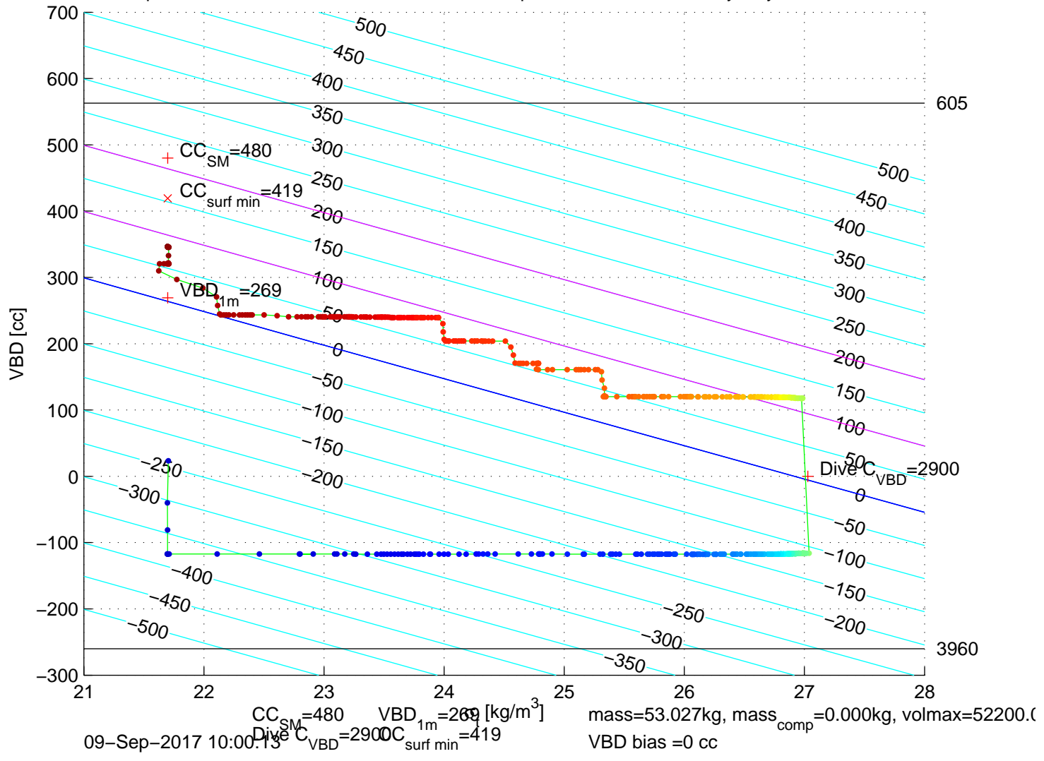
p6300434: SG630 Mission 7 Jul 2017 09-Sep-2017 09:08:36Z – buoyancy contoured
