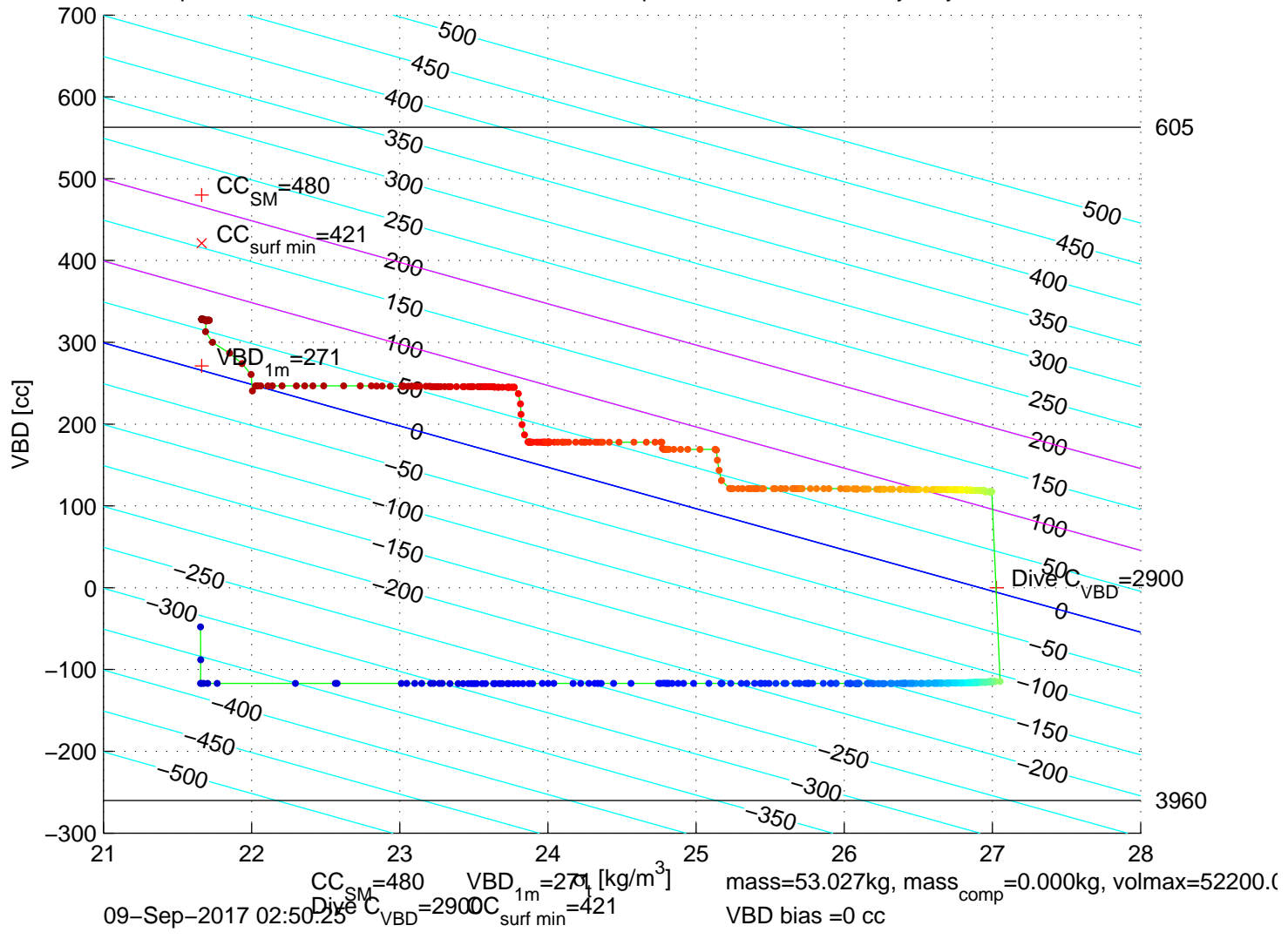
p6300432: SG630 Mission 7 Jul 2017 09-Sep-2017 04:26:36Z – buoyancy contoured
