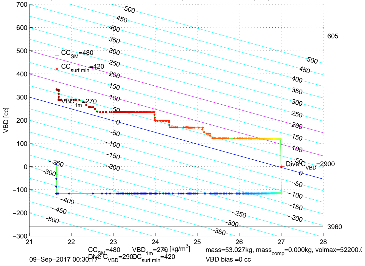
p6300431: SG630 Mission 7 Jul 2017 09-Sep-2017 01:55:52Z – buoyancy contoured
