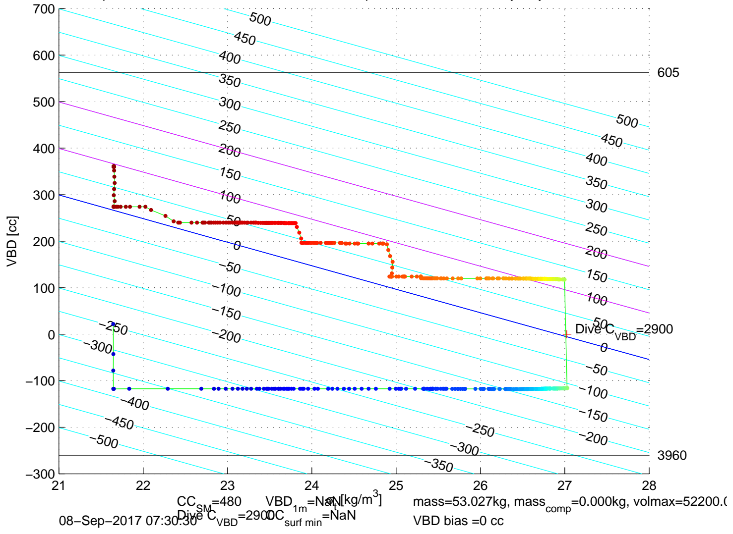
p6300424: SG630 Mission 7 Jul 2017 08-Sep-2017 08:54:53Z – buoyancy contoured
