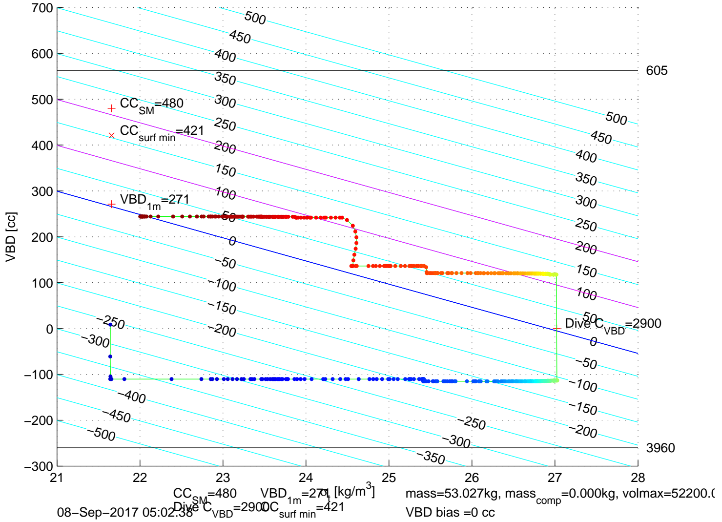
p6300423: SG630 Mission 7 Jul 2017 08-Sep-2017 06:38:11Z – buoyancy contoured
