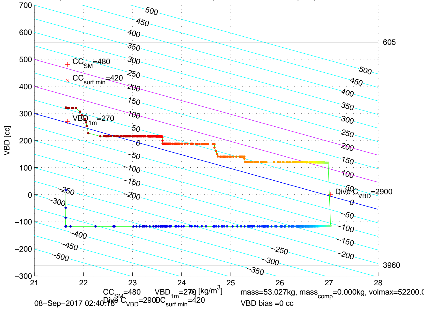
p6300422: SG630 Mission 7 Jul 2017 08-Sep-2017 04:15:49Z – buoyancy contoured
