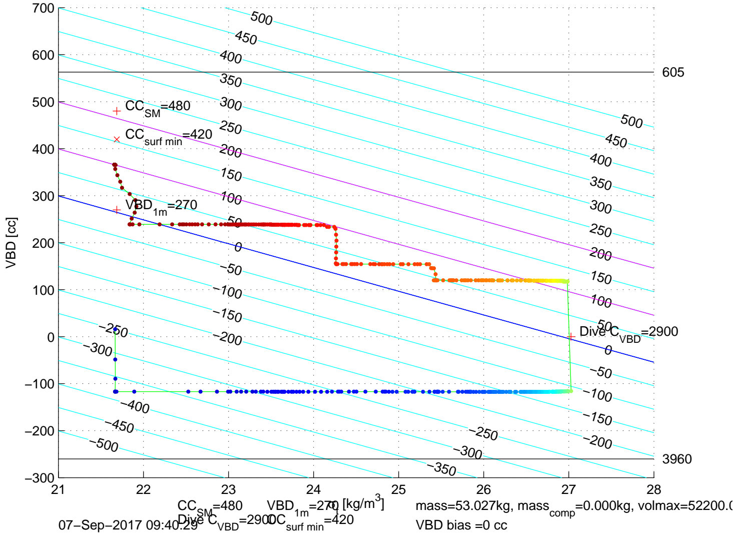
p6300415: SG630 Mission 7 Jul 2017 07-Sep-2017 11:06:43Z – buoyancy contoured
