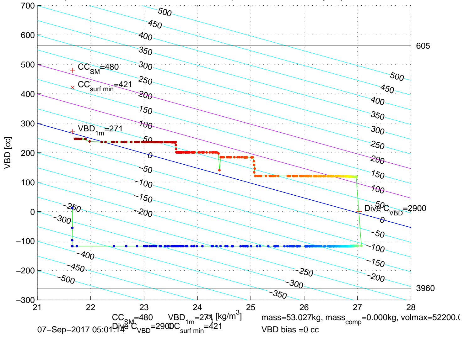
p6300413: SG630 Mission 7 Jul 2017 07-Sep-2017 06:29:46Z – buoyancy contoured
