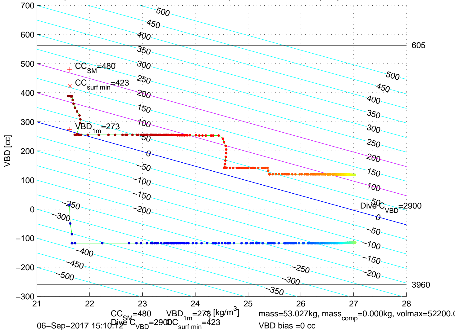
p6300407: SG630 Mission 7 Jul 2017 06-Sep-2017 16:49:06Z – buoyancy contoured
