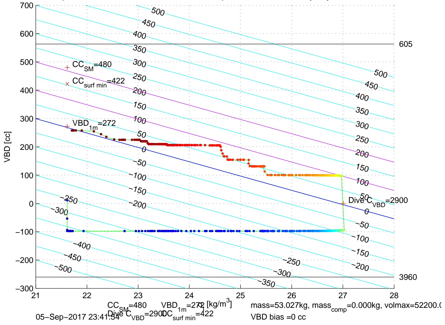
p6300401: SG630 Mission 7 Jul 2017 06-Sep-2017 00:57:16Z – buoyancy contoured
