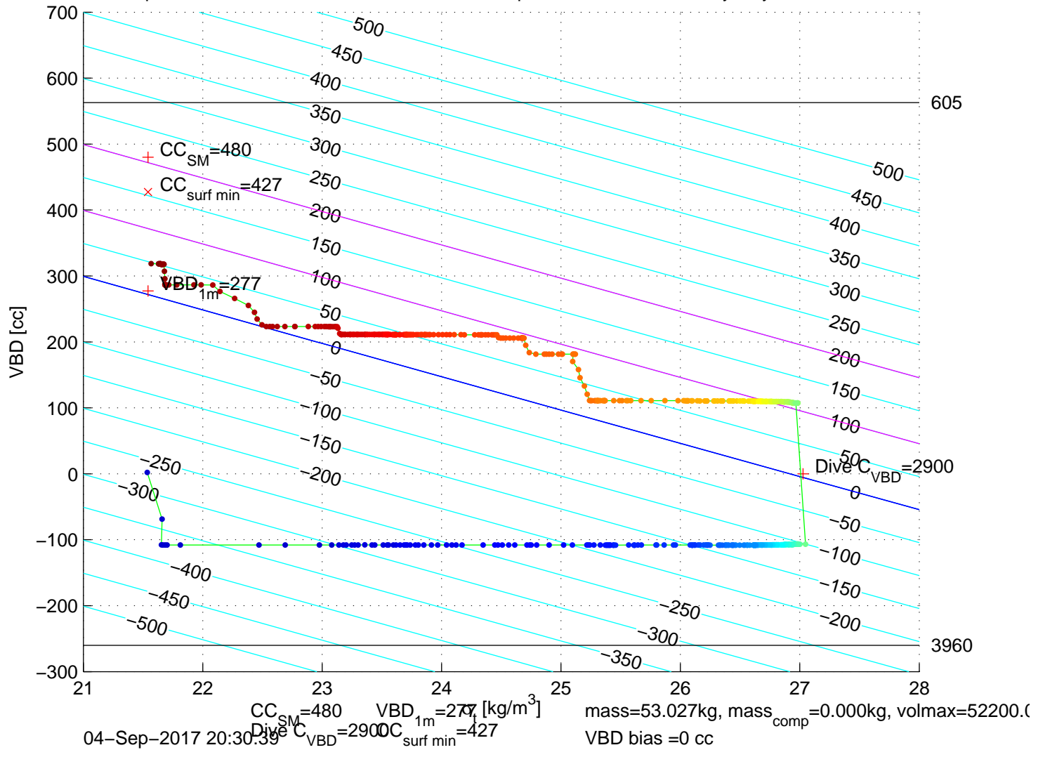
p6300390: SG630 Mission 7 Jul 2017 04-Sep-2017 21:57:46Z – buoyancy contoured
