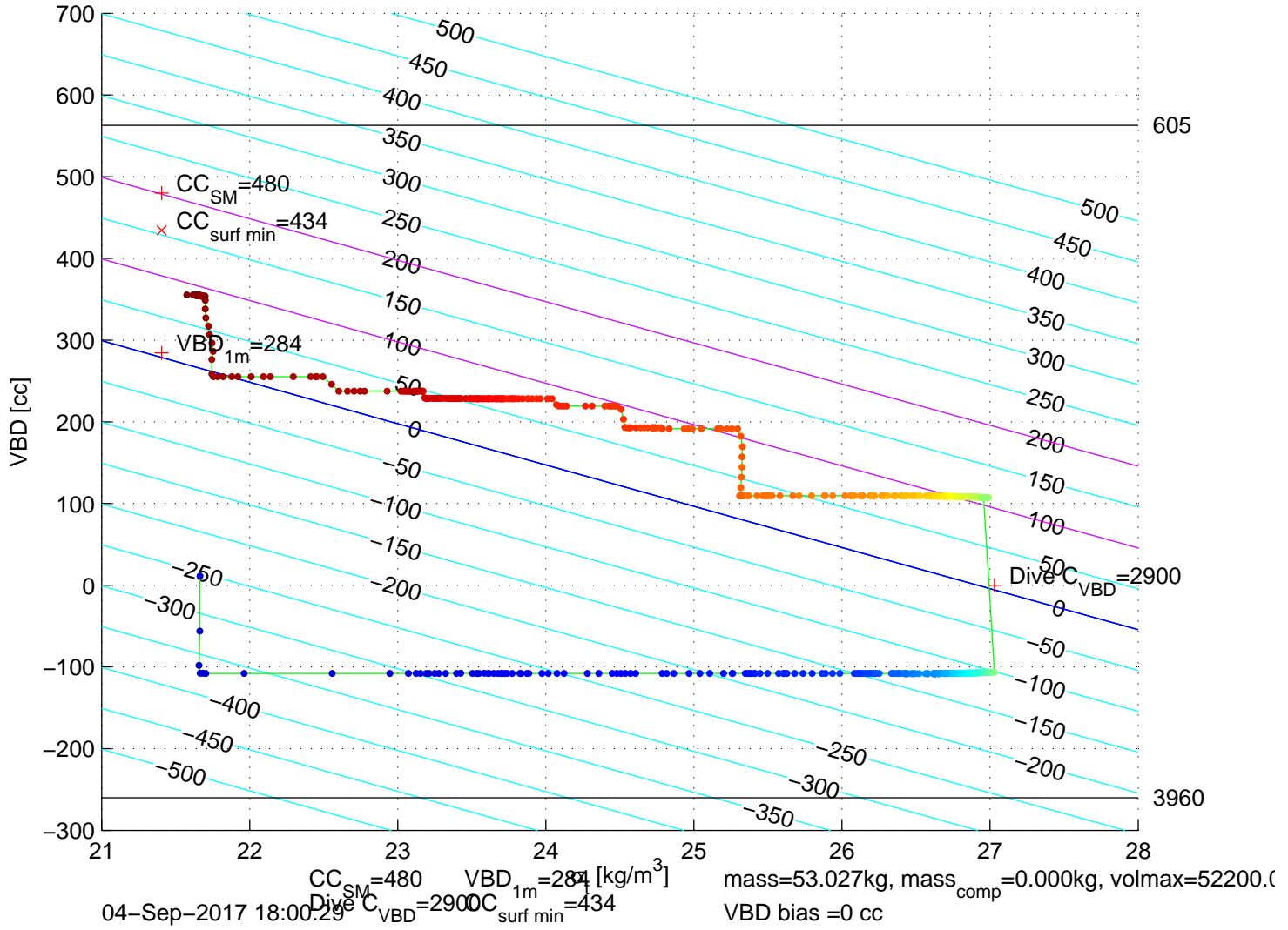
p6300389: SG630 Mission 7 Jul 2017 04-Sep-2017 19:34:12Z – buoyancy contoured
