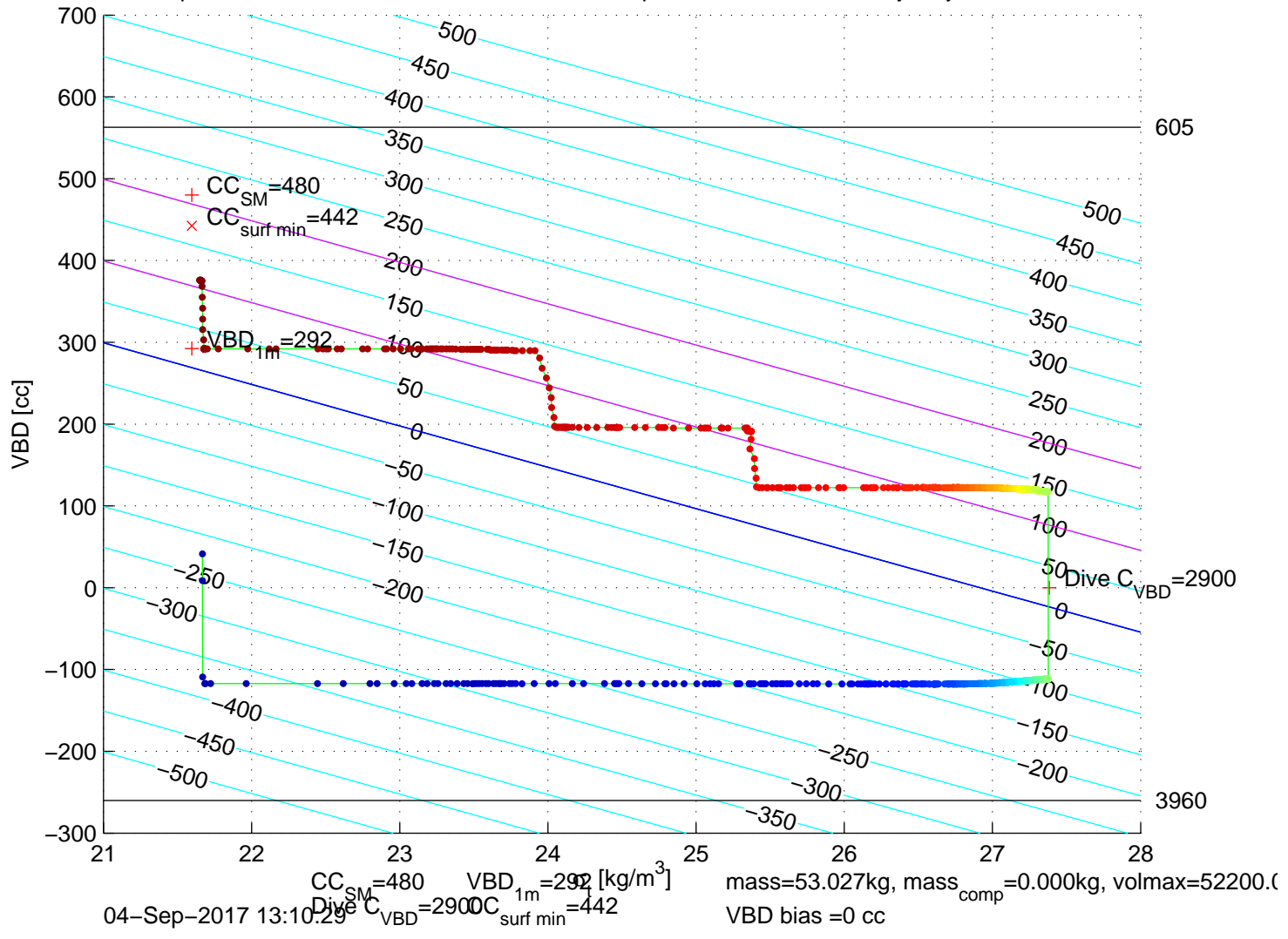
p6300386: SG630 Mission 7 Jul 2017 04-Sep-2017 10:31:03Z – buoyancy contoured
