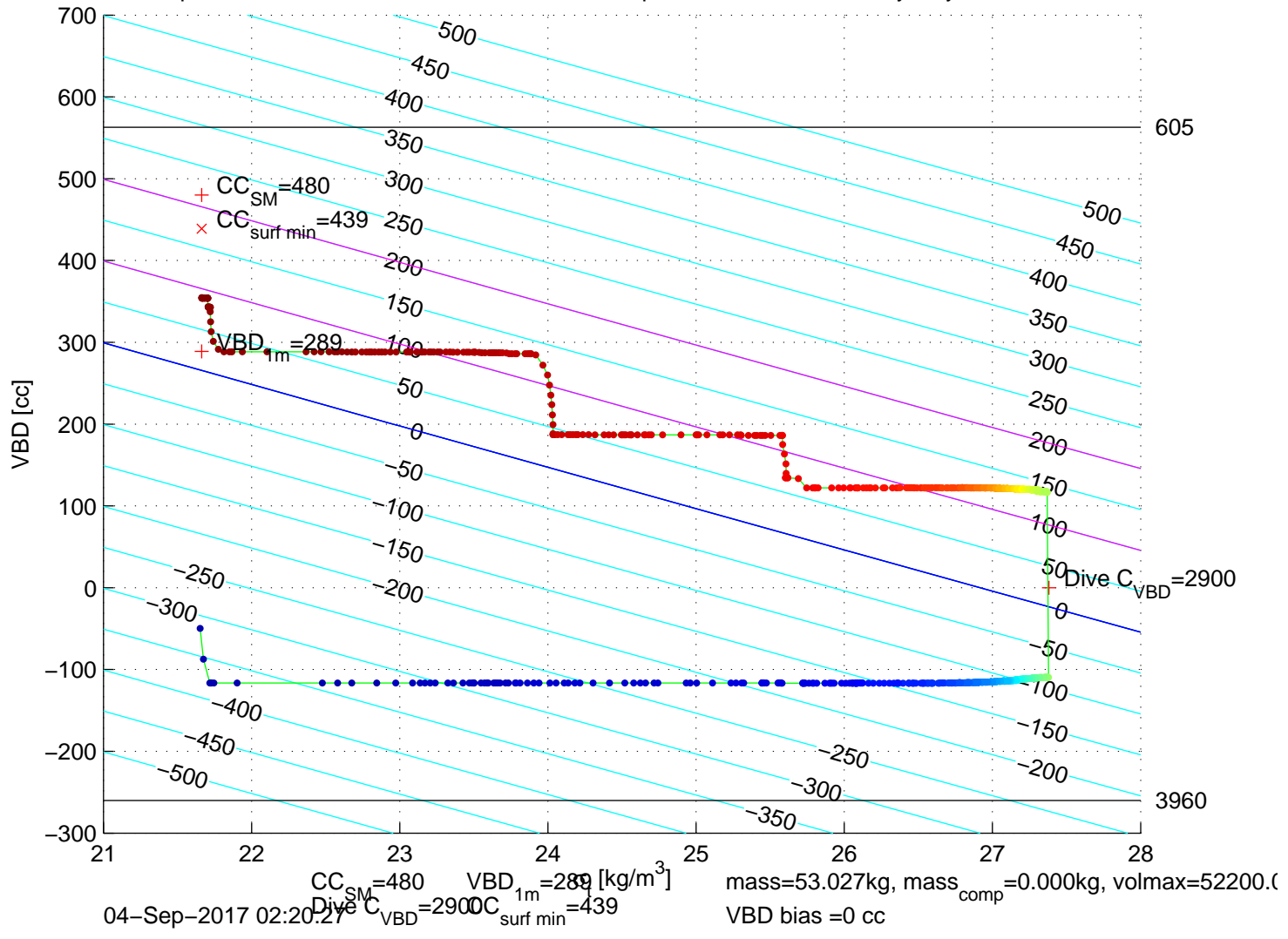
p6300384: SG630 Mission 7 Jul 2017 04-Sep-2017 01:48:37Z – buoyancy contoured
