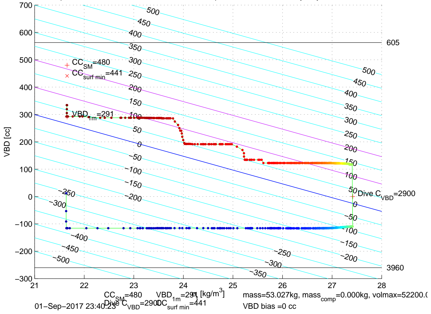
p6300372: SG630 Mission 7 Jul 2017 01-Sep-2017 23:15:20Z – buoyancy contoured
