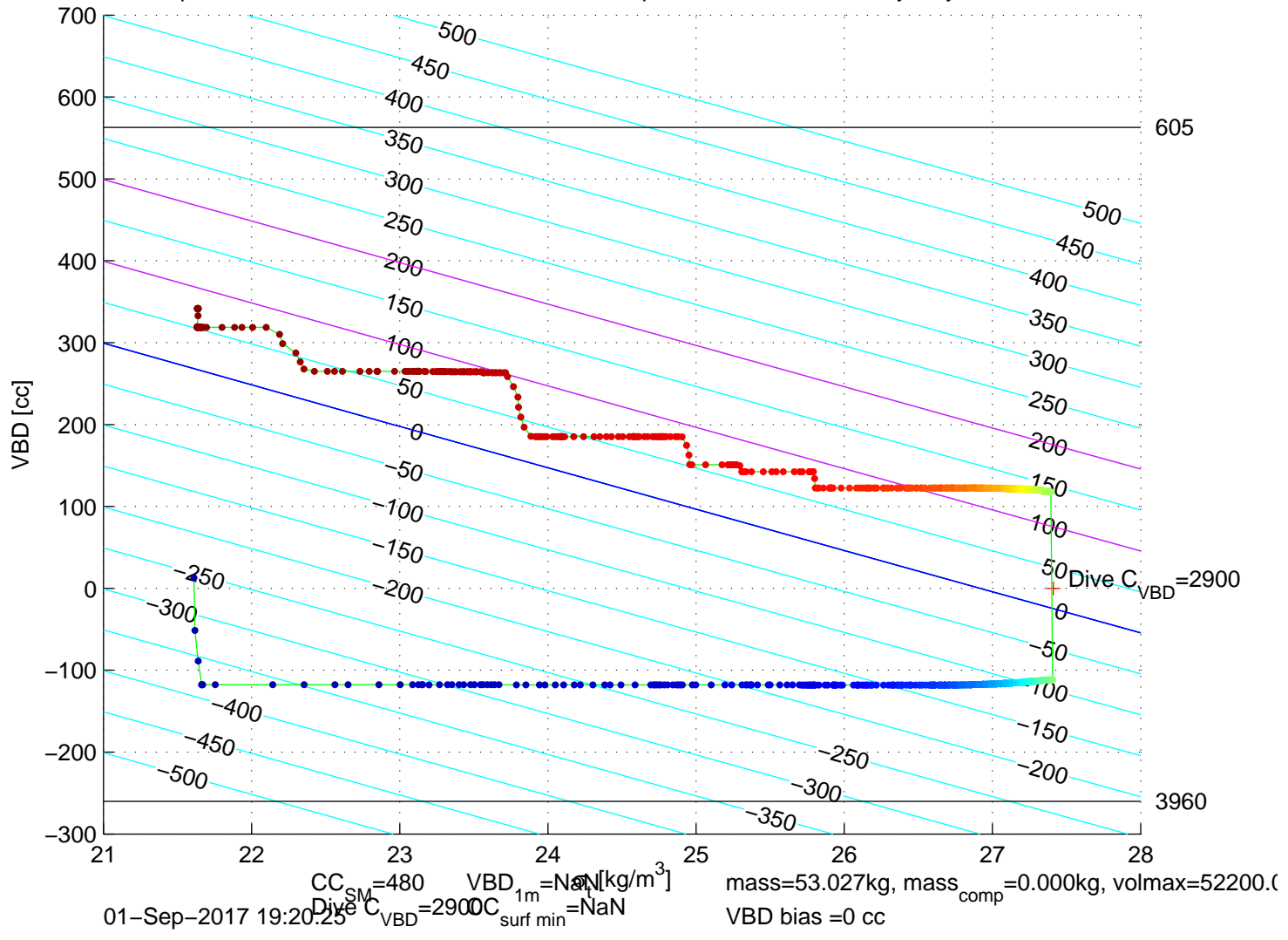
p6300371: SG630 Mission 7 Jul 2017 01-Sep-2017 18:58:09Z – buoyancy contoured
