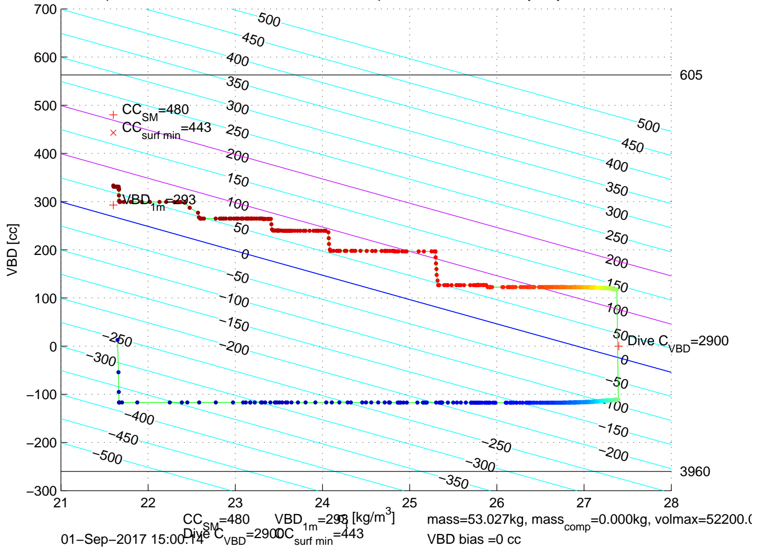
p6300370: SG630 Mission 7 Jul 2017 01-Sep-2017 14:44:59Z – buoyancy contoured
