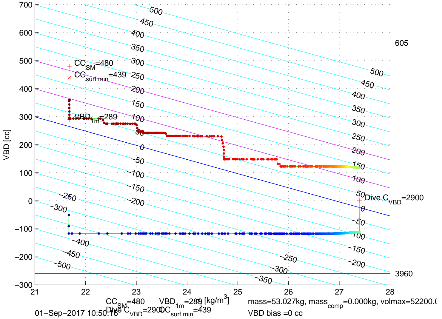
p6300368: SG630 Mission 7 Jul 2017 01-Sep-2017 06:19:05Z – buoyancy contoured
