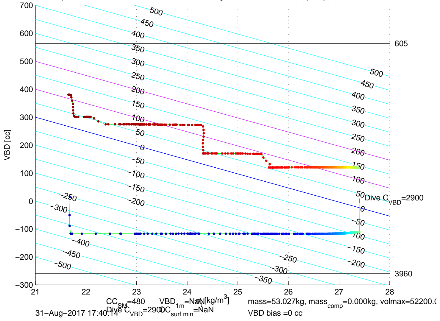
p6300365: SG630 Mission 7 Jul 2017 31-Aug-2017 17:24:08Z – buoyancy contoured
