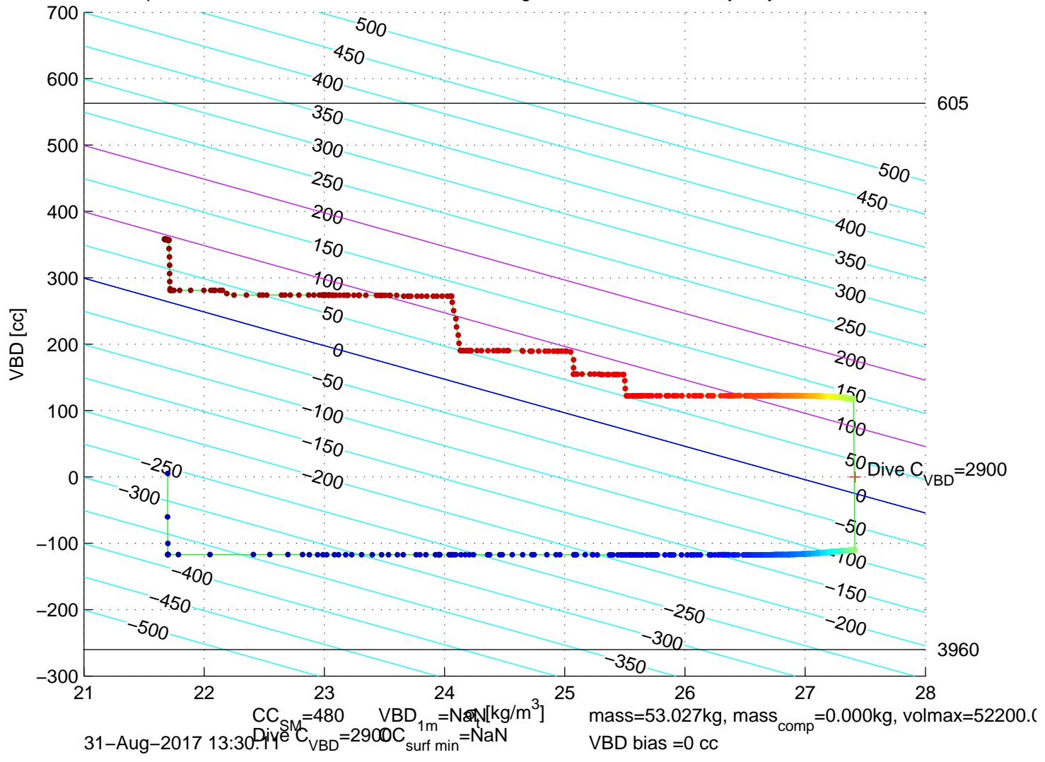
p6300364: SG630 Mission 7 Jul 2017 31-Aug-2017 13:10:59Z – buoyancy contoured
