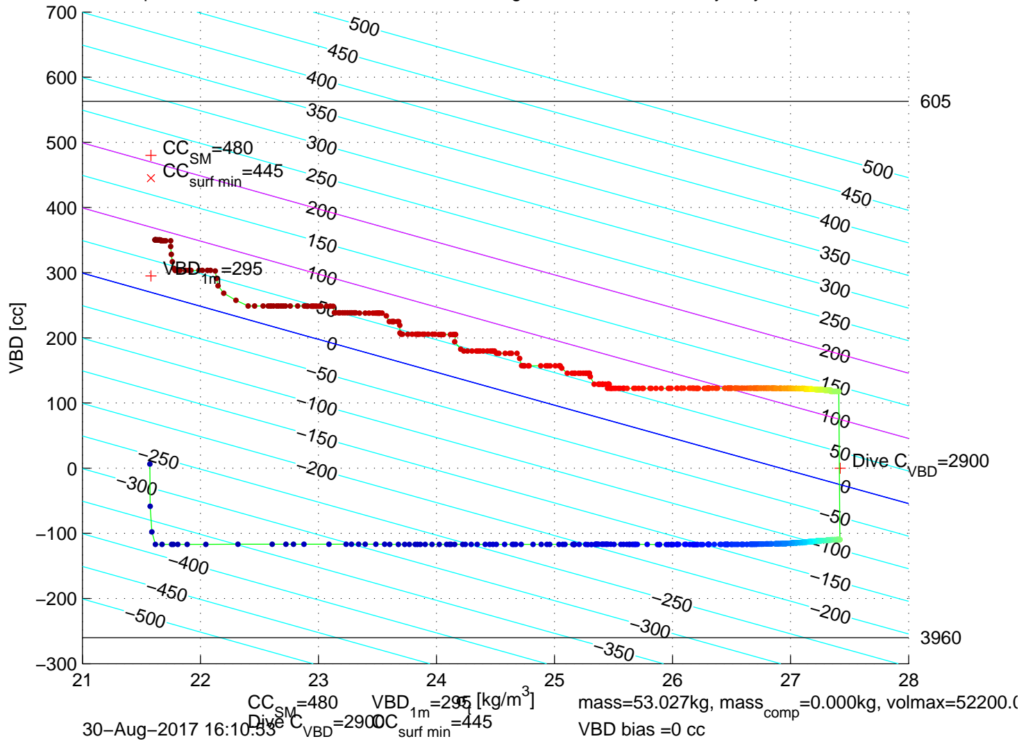
p6300359: SG630 Mission 7 Jul 2017 30-Aug-2017 15:39:32Z – buoyancy contoured
