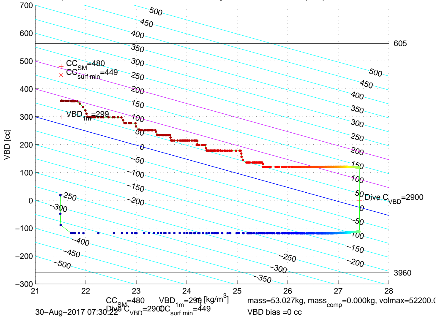
p6300357: SG630 Mission 7 Jul 2017 30-Aug-2017 07:18:30Z – buoyancy contoured
