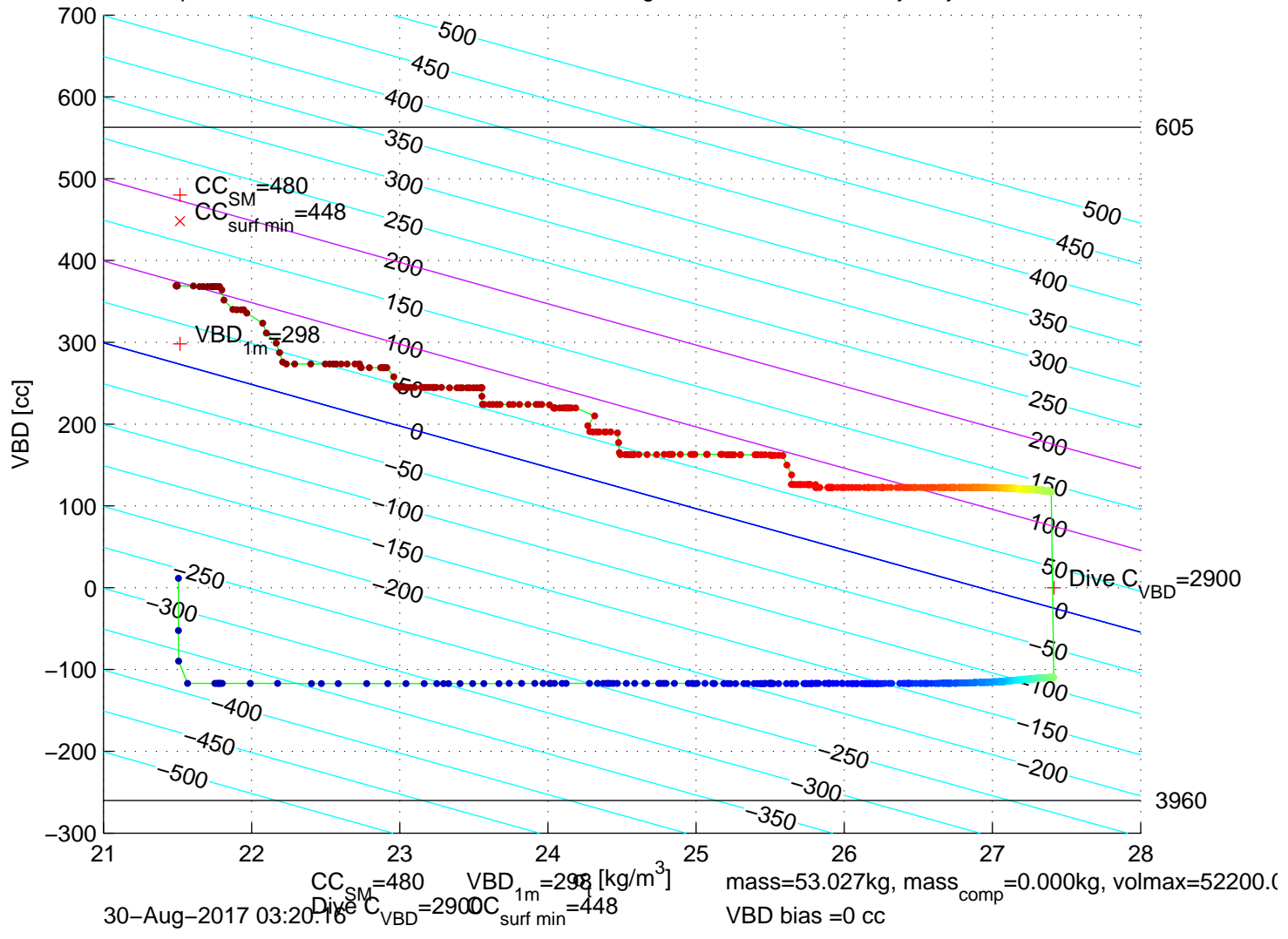
p6300356: SG630 Mission 7 Jul 2017 30-Aug-2017 03:13:41Z – buoyancy contoured
