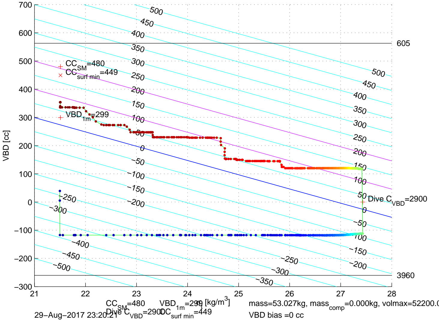
p6300355: SG630 Mission 7 Jul 2017 29-Aug-2017 22:58:06Z – buoyancy contoured
