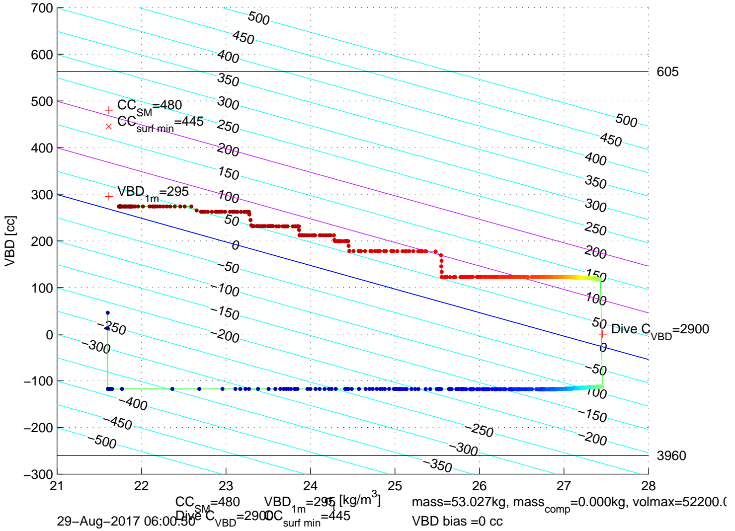
p6300351: SG630 Mission 7 Jul 2017 29-Aug-2017 05:44:26Z – buoyancy contoured
