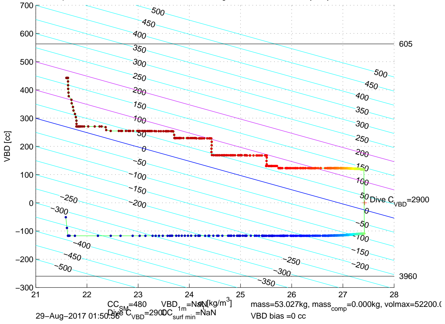
p6300350: SG630 Mission 7 Jul 2017 29-Aug-2017 01:36:54Z – buoyancy contoured
