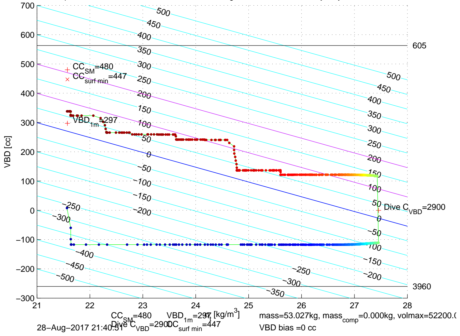
p6300349: SG630 Mission 7 Jul 2017 28-Aug-2017 21:09:50Z – buoyancy contoured
