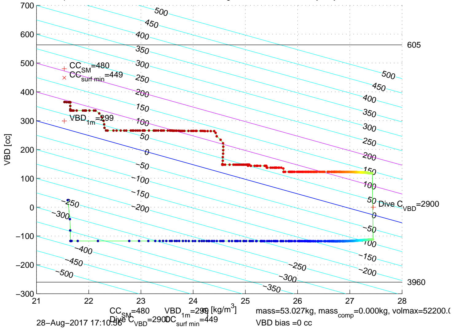
p6300348: SG630 Mission 7 Jul 2017 28-Aug-2017 17:01:54Z – buoyancy contoured
