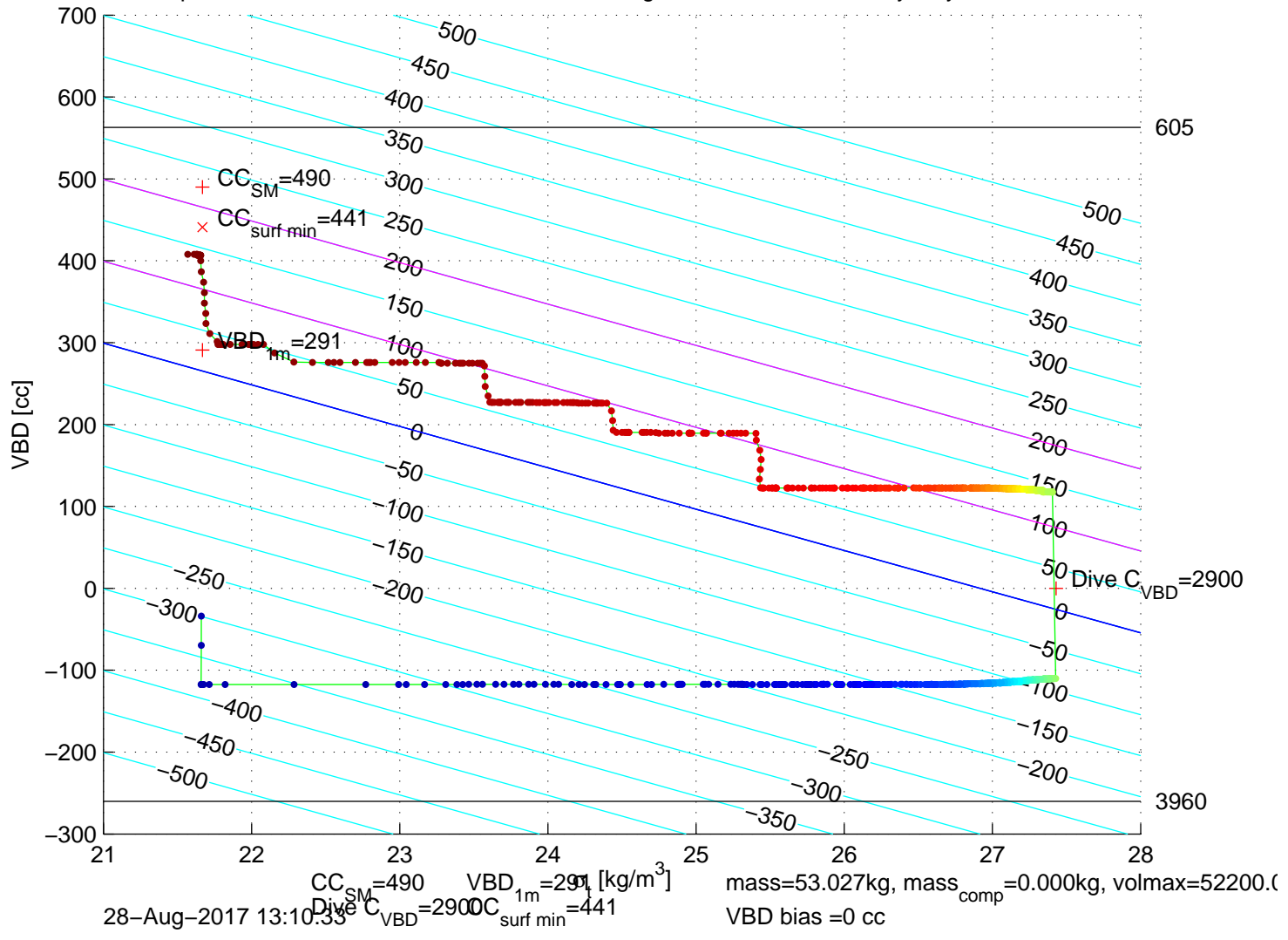
p6300347: SG630 Mission 7 Jul 2017 28-Aug-2017 12:54:23Z – buoyancy contoured
