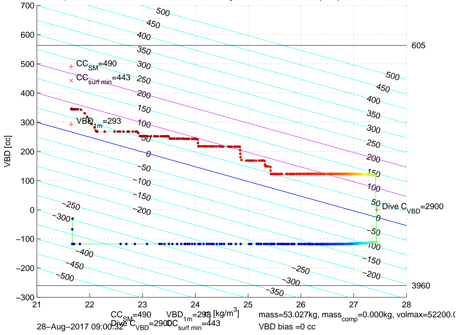
p6300346: SG630 Mission 7 Jul 2017 28-Aug-2017 08:39:39Z – buoyancy contoured
