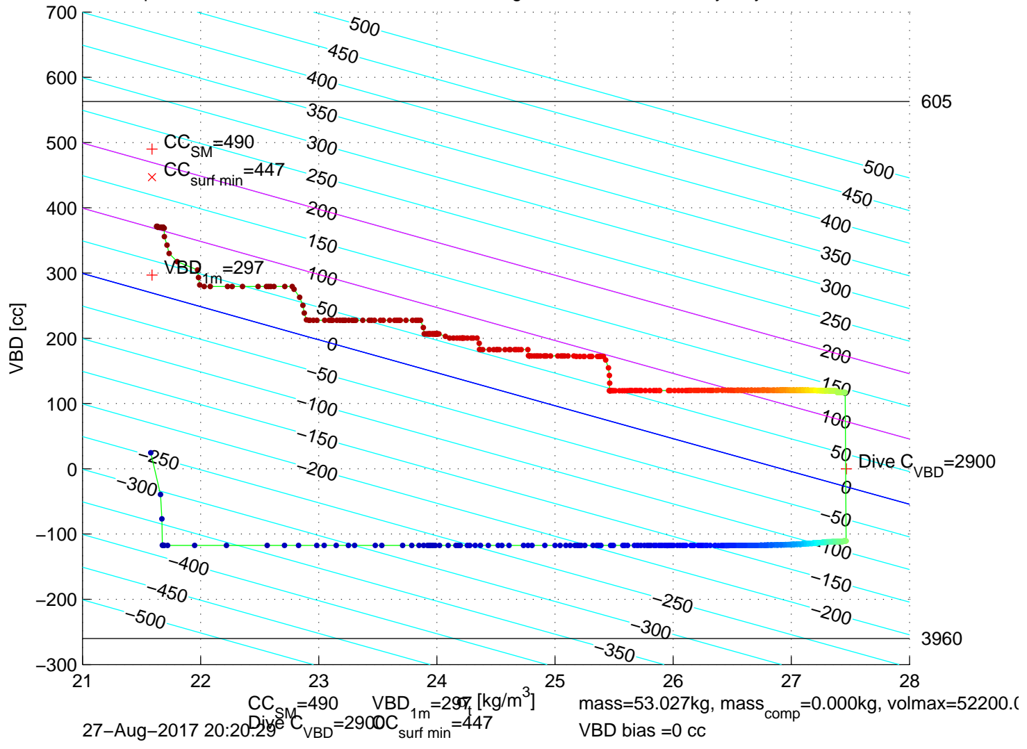
p6300343: SG630 Mission 7 Jul 2017 27-Aug-2017 20:00:58Z – buoyancy contoured
