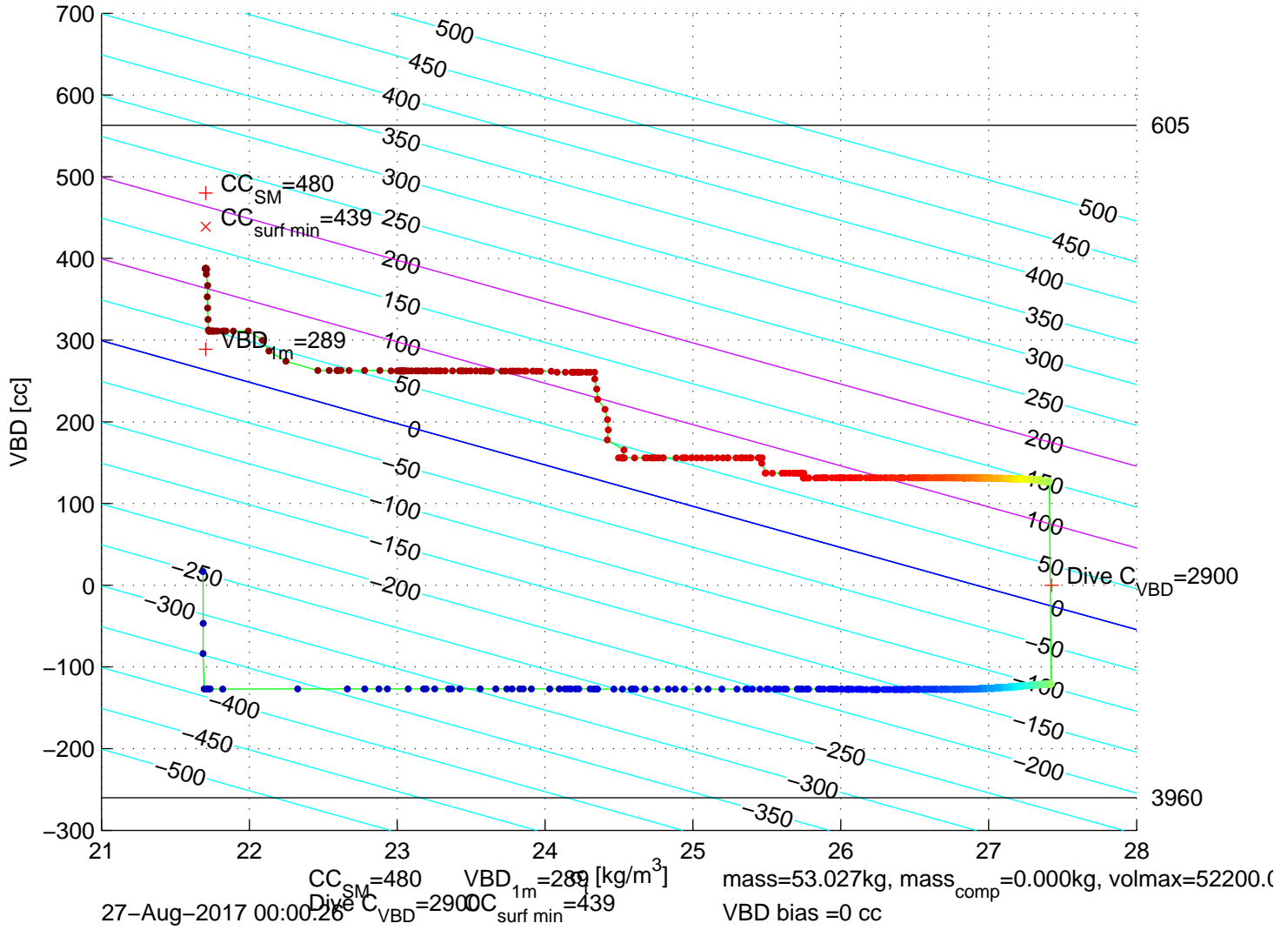
p6300338: SG630 Mission 7 Jul 2017 26–Aug–2017 23:59:43Z – buoyancy contoured
