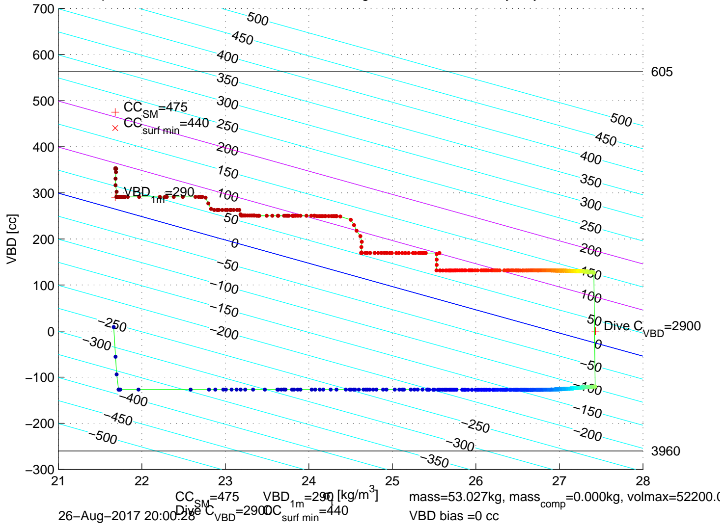
p6300337: SG630 Mission 7 Jul 2017 26-Aug-2017 19:53:14Z – buoyancy contoured
