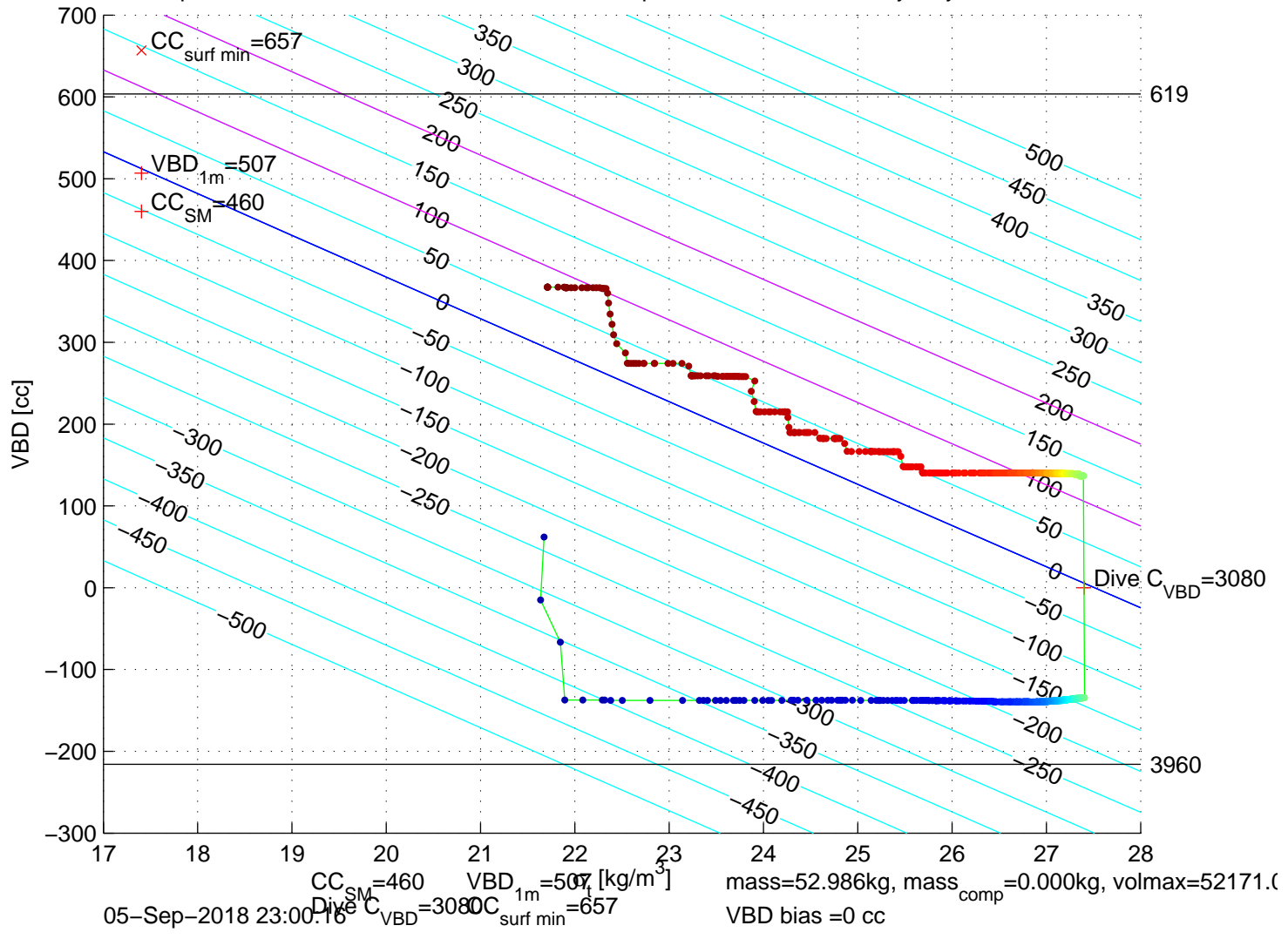
p6300335: SG630 Mission 8 Jul 2018 05-Sep-2018 23:09:23Z - buoyancy contoured
