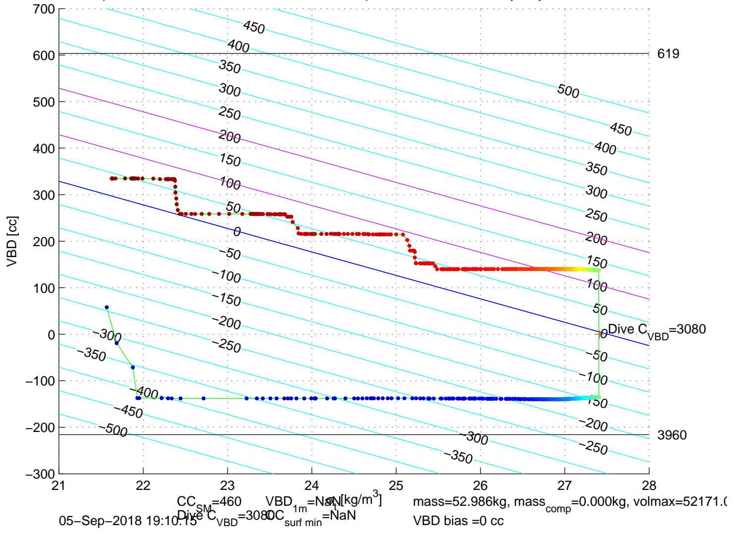
p6300334: SG630 Mission 8 Jul 2018 05-Sep-2018 19:24:21Z - buoyancy contoured
