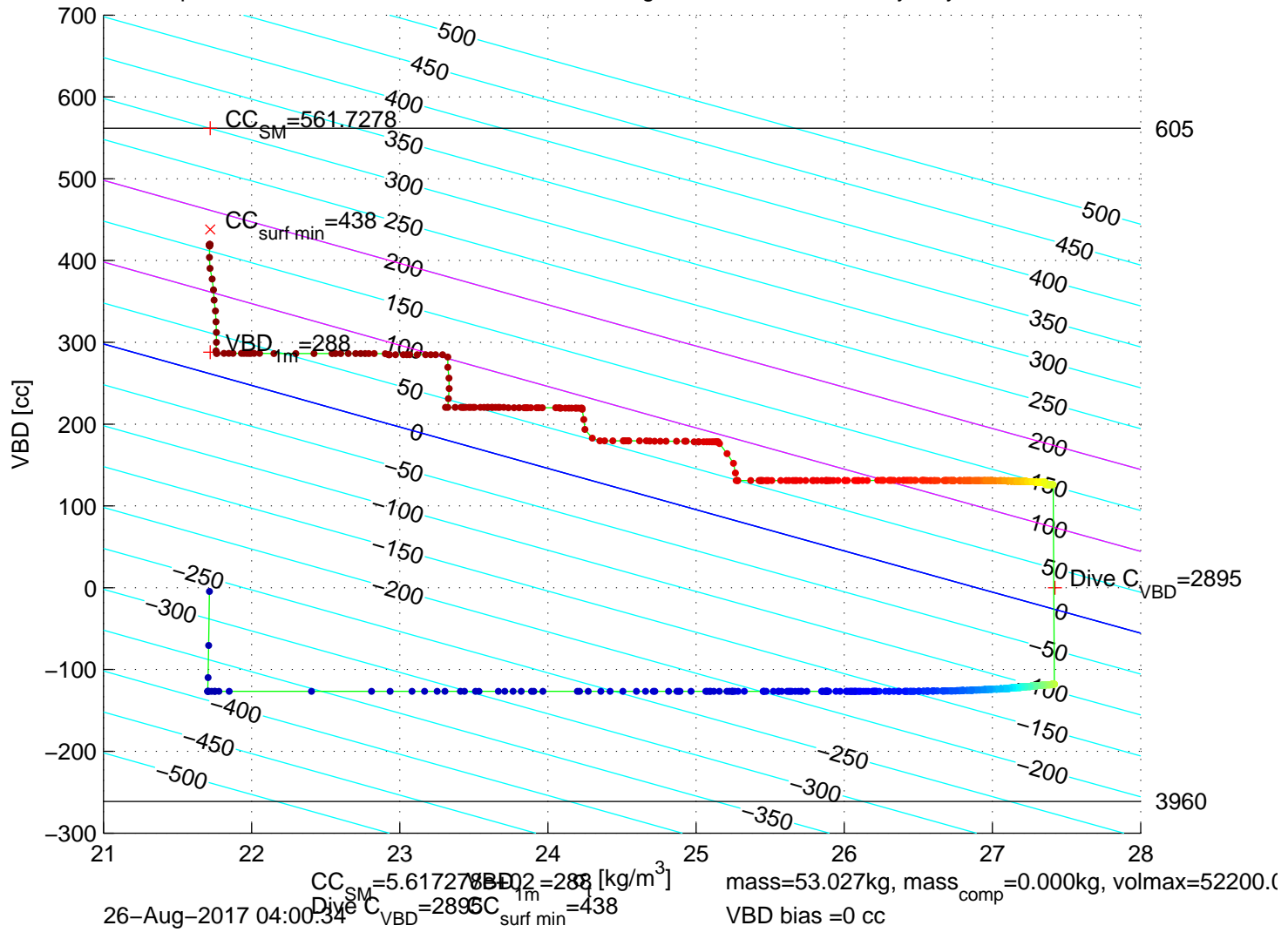
p6300333: SG630 Mission 7 Jul 2017 26-Aug-2017 03:40:00Z – buoyancy contoured
