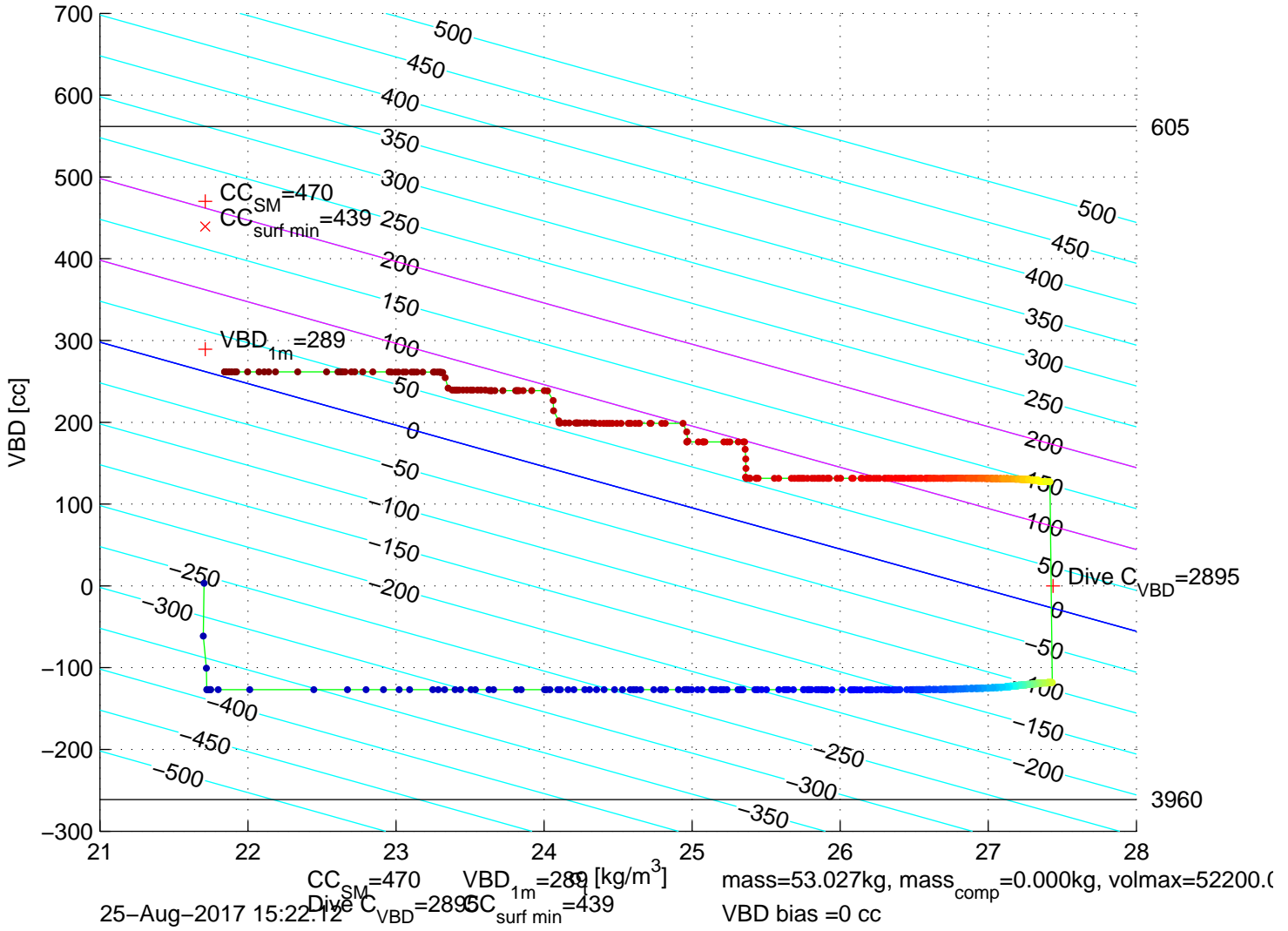
p6300330: SG630 Mission 7 Jul 2017 25-Aug-2017 15:09:17Z – buoyancy contoured
