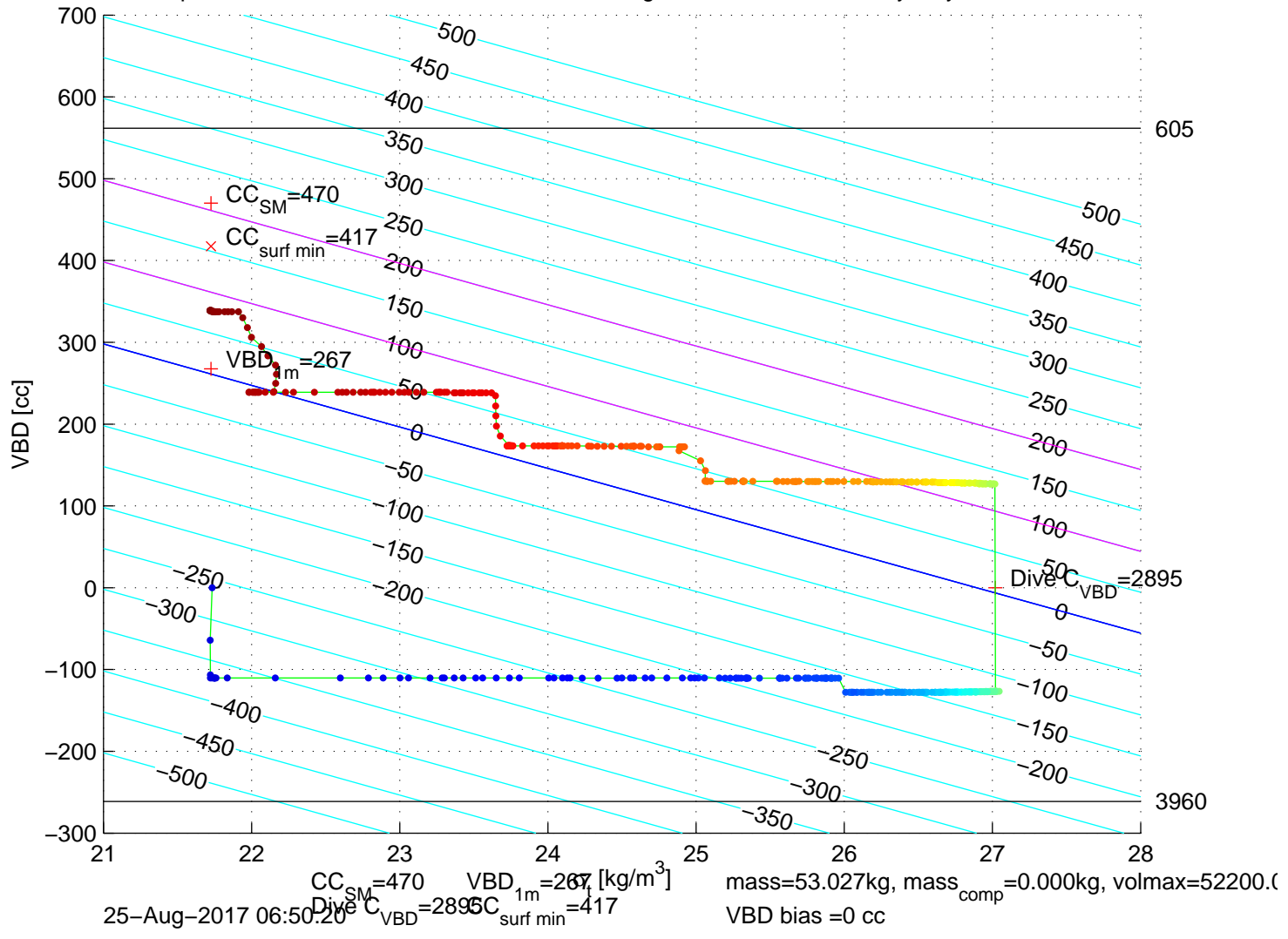
p6300327: SG630 Mission 7 Jul 2017 25-Aug-2017 08:26:15Z – buoyancy contoured
