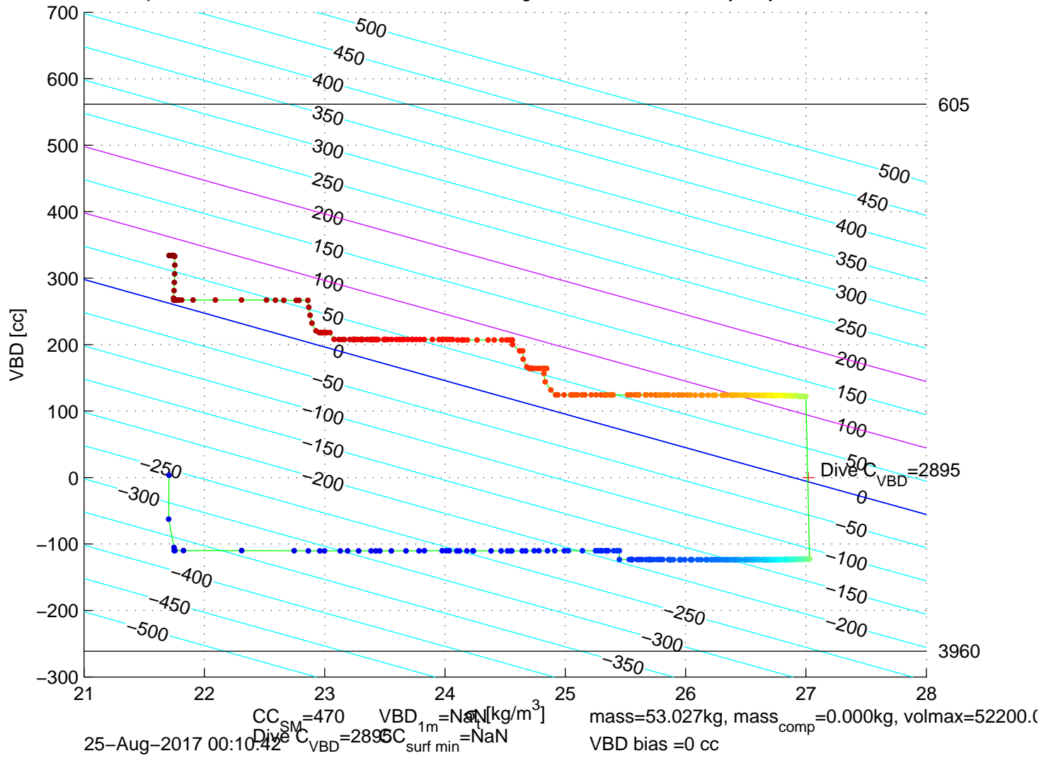
p6300324: SG630 Mission 7 Jul 2017 25-Aug-2017 02:09:11Z – buoyancy contoured
