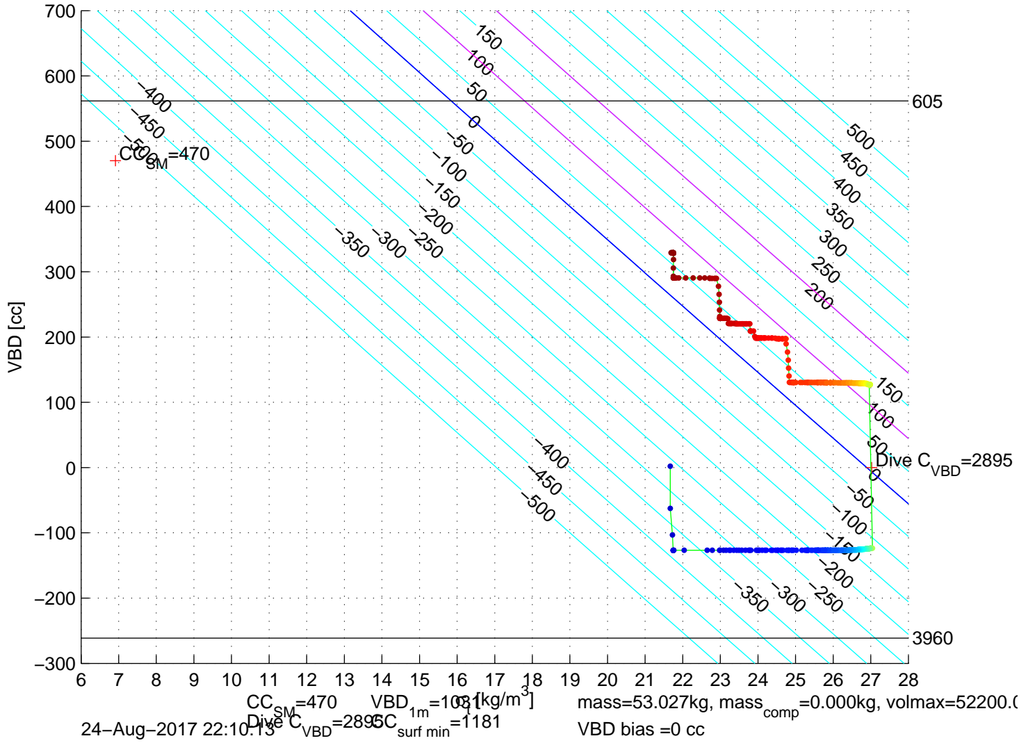
p6300323: SG630 Mission 7 Jul 2017 24-Aug-2017 23:54:41Z – buoyancy contoured
