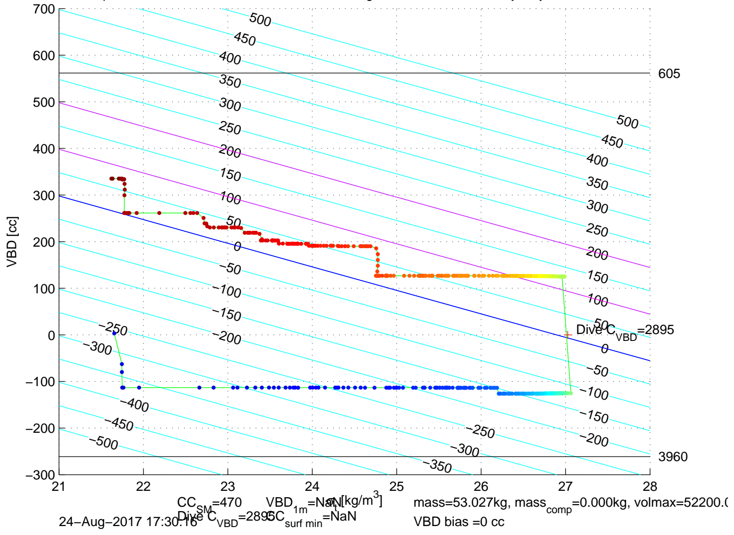
p6300321: SG630 Mission 7 Jul 2017 24-Aug-2017 19:23:00Z – buoyancy contoured
