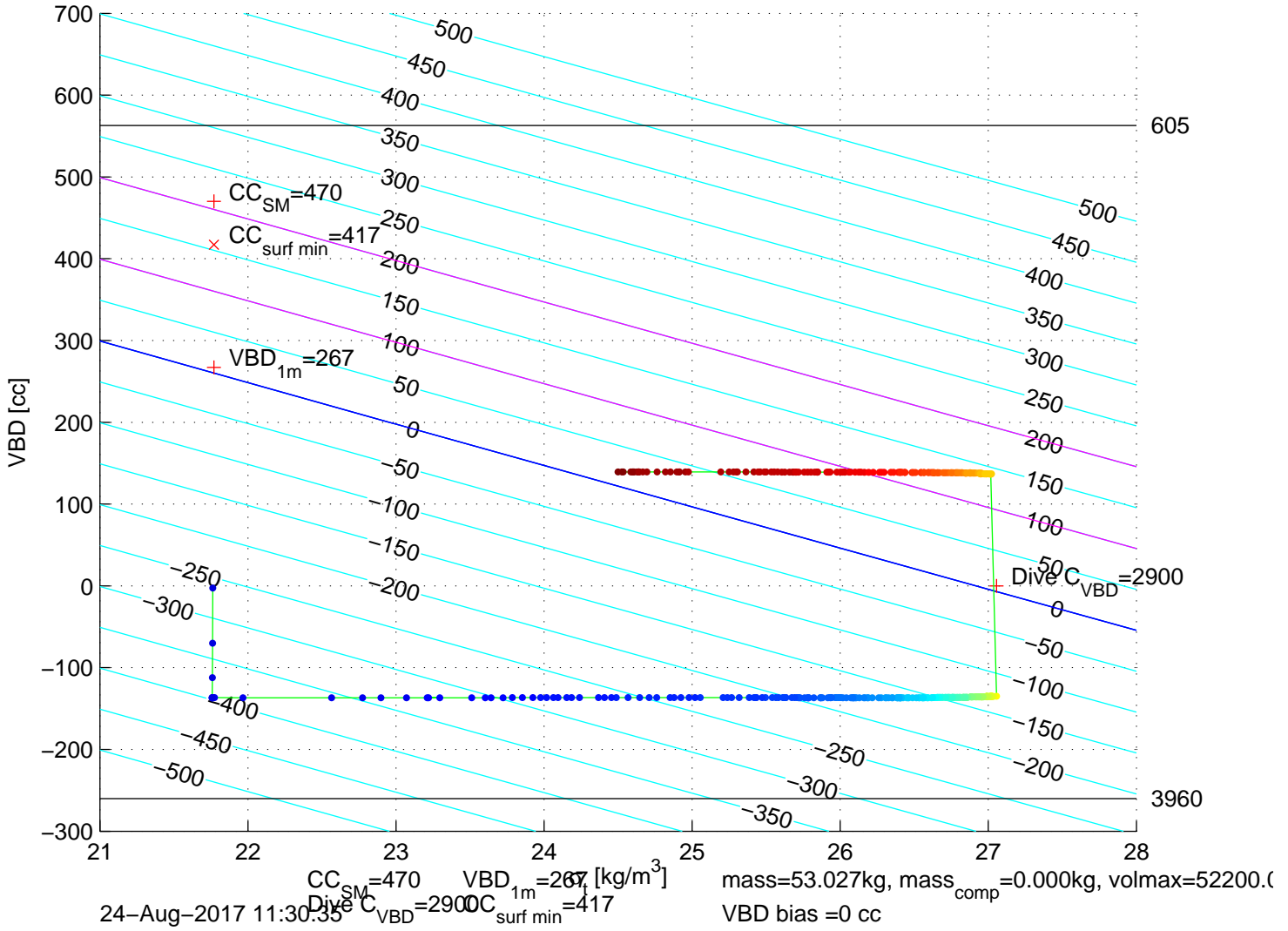
p6300318: SG630 Mission 7 Jul 2017 24-Aug-2017 13:11:05Z – buoyancy contoured
