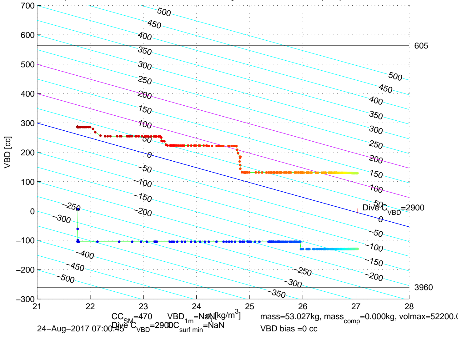
p6300316: SG630 Mission 7 Jul 2017 24-Aug-2017 08:54:36Z – buoyancy contoured
