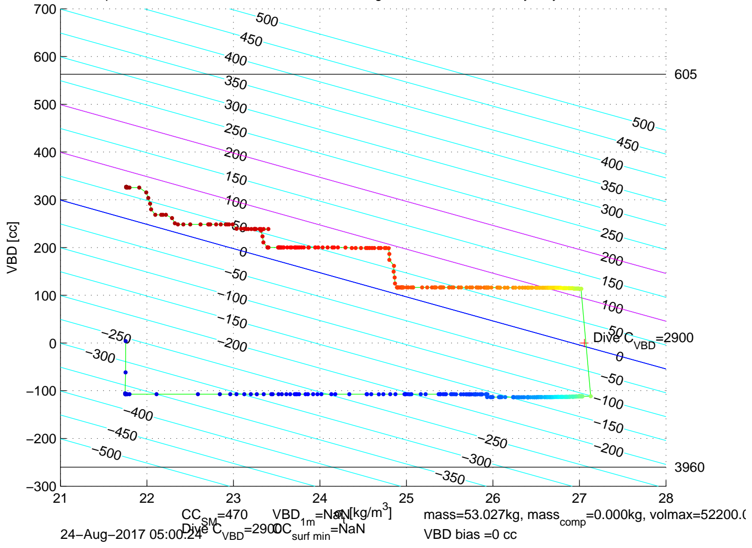
p6300315: SG630 Mission 7 Jul 2017 24-Aug-2017 06:51:01Z – buoyancy contoured
