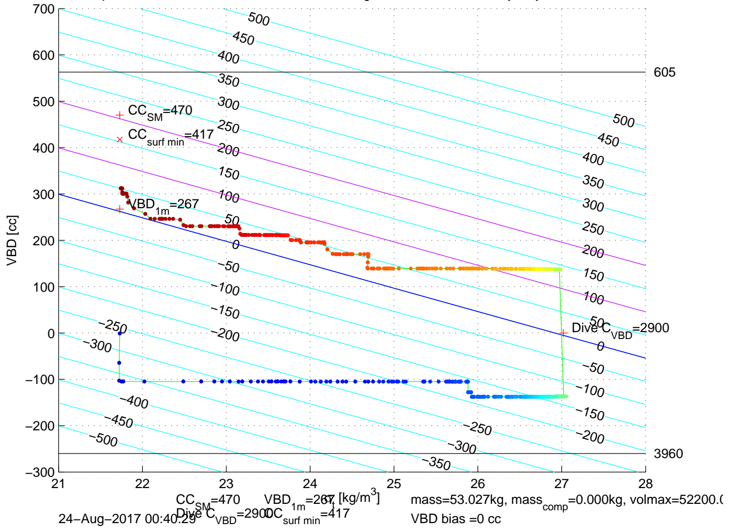
p6300313: SG630 Mission 7 Jul 2017 24-Aug-2017 02:44:08Z – buoyancy contoured
